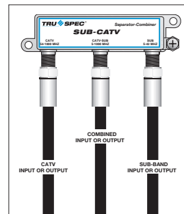
Connection Diagram
