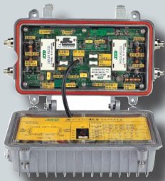
Trunk Amplifiers
