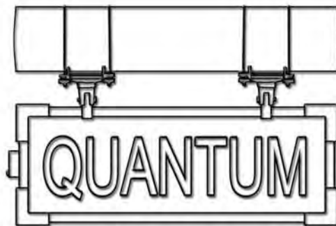
SUSPENDED MOUNT ILLUMINATED SIGNS
