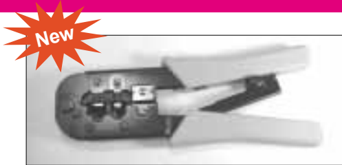
MCT-3 DELUXE MODULAR RATCHET CRIMPING TOOL Cut, Strip and Crimp, Metal Construction For 8P8C/RJ-45, 6P4C/RJ-11
