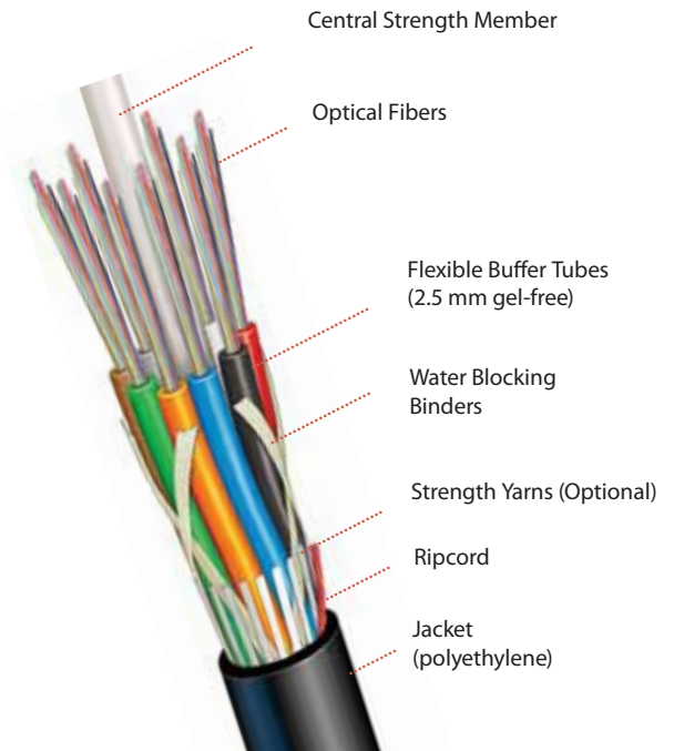
Dielectric Loose Tube
