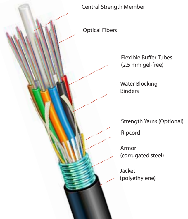
Armored Loose Tube (SP)
