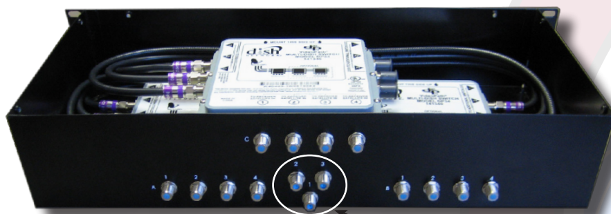
Rear of assembled unit with lid removed — Three Satellite Inputs
